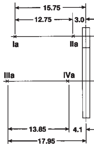
Fig. 9 Overhung Mounting
