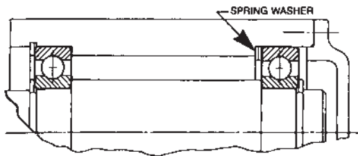
MOUNTING WITH SNAP-RINGS AND SPRING WASHER
