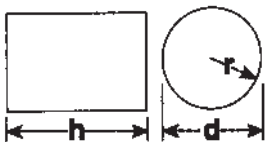
Cylinder
