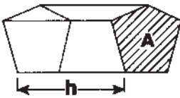
Prism
