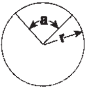
Spherical Wedge
