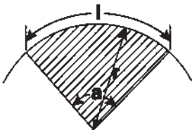
Circular Sector
