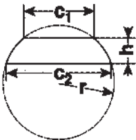
Spherical Zone
