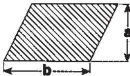
Parallelogram
