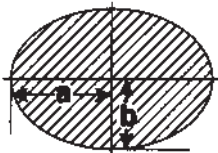
Ellipse
