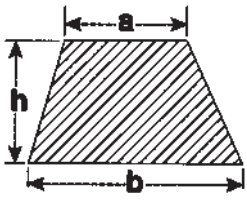
Trapezoid
