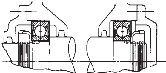
STANDARD MOUNTING
