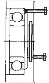
Housing with tapped holes for withdrawal screws
