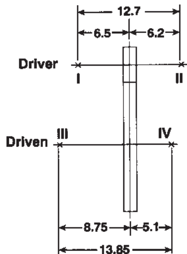
Fig. 8 Straddle Mounting
