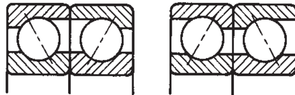
Face-to-face Back-to-back Figure 4 Angular contact ball bearings pair mounting arrangements.
