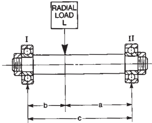
Fig. 3 Straddle Mounting
