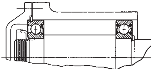
MOUNTING WITH LOCK NUT AND SNAP-RING
