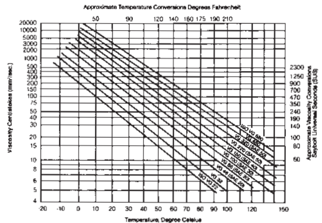
Figure 2 Viscosity-Temperature Chart
