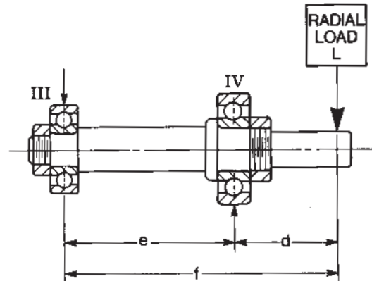
Fig. 4 Overhung Mounting
