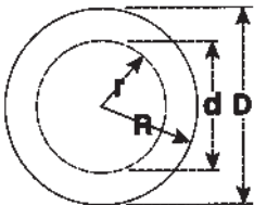
Hollow Sphere
