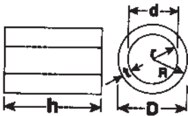
Hollow Cylinder
