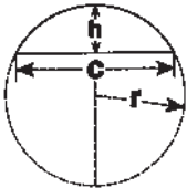
Spherical Segment
